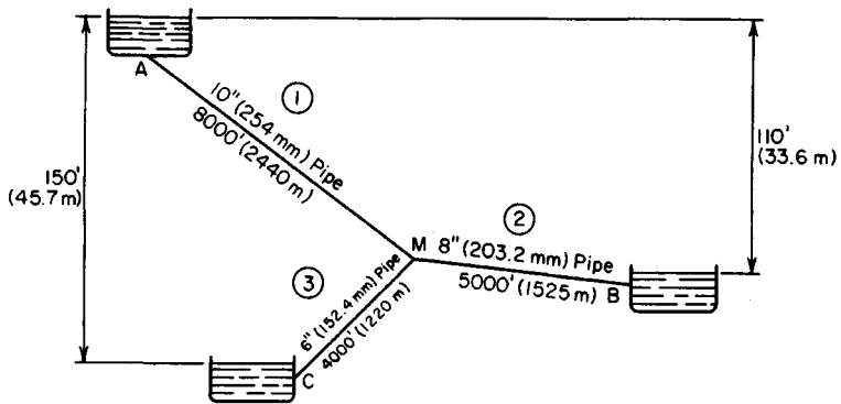
FIGURE 9. Branching pipes.
