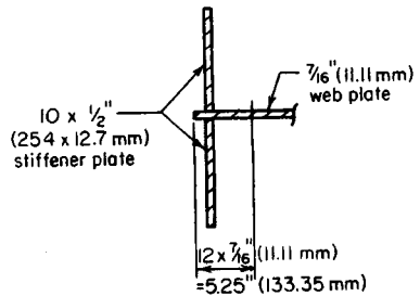
FIGURE 9. Effective column section.
