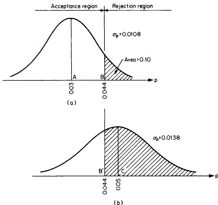
FIGURE 25. Sampling distribution of proportion of defective units.
