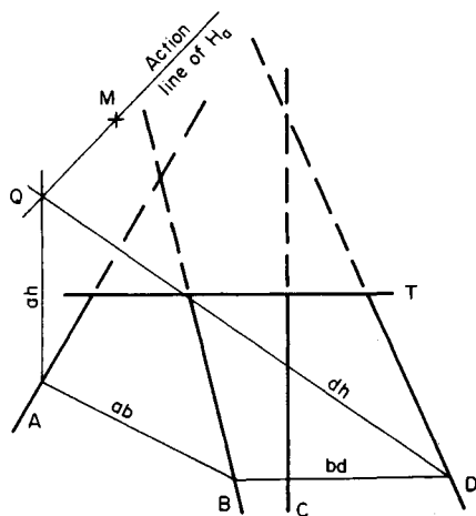
(c) Construction to locate action line of H_a
