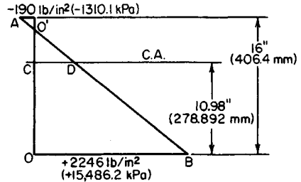
FIGURE 40. Prestress diagram.
