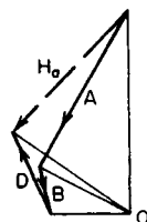
(b) Force polygon for H_a
