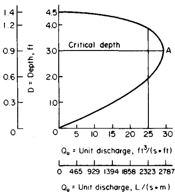
(a) Diagram for H_e = 4.5 \text{ ft} ( 1.4 \text{ m} )
