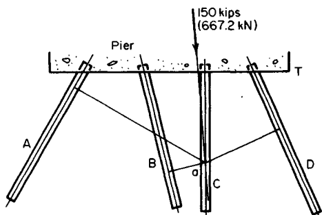
(a) Pile group and load
