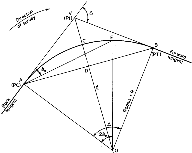
FIGURE 13. Circular curve.
