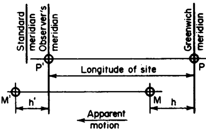
FIGURE 12. Culmination of Polaris.
