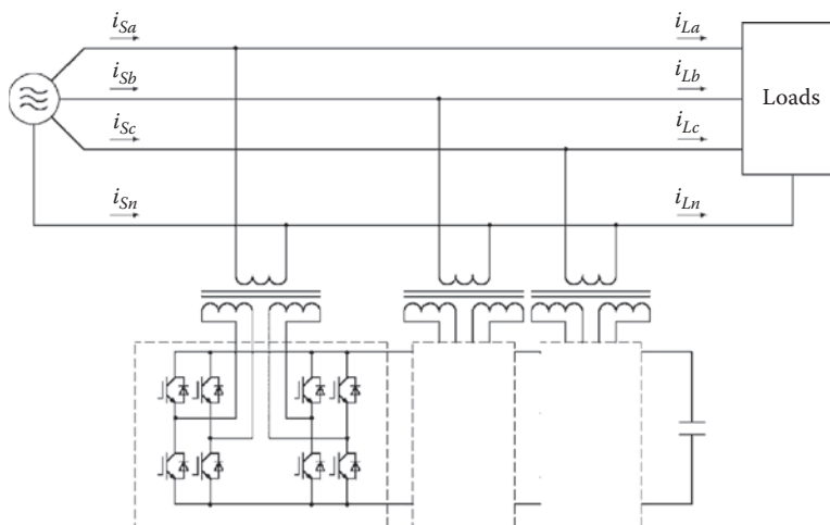
FIGURE 26.15 Shunt active filter for three-phase four-wire system.
