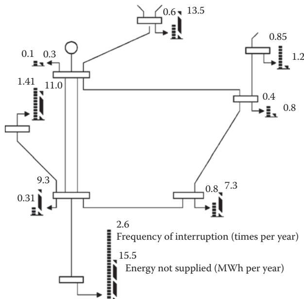
FIGURE 17.1 Prediction of supply point reliability.
