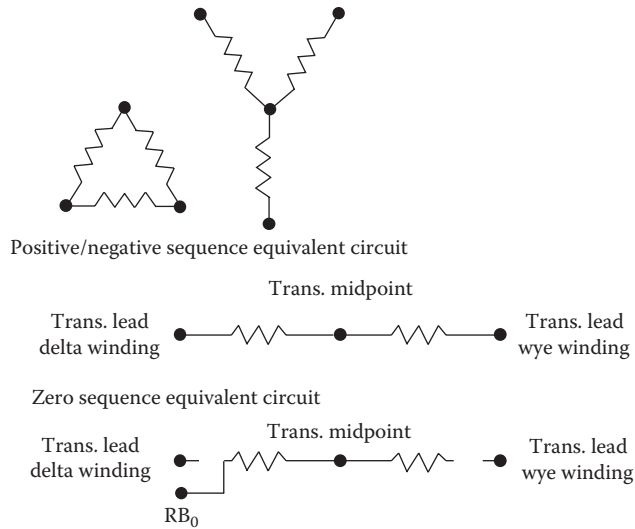
FIGURE 2.19 Transformer equivalent circuits, windings connected delta-wye.
