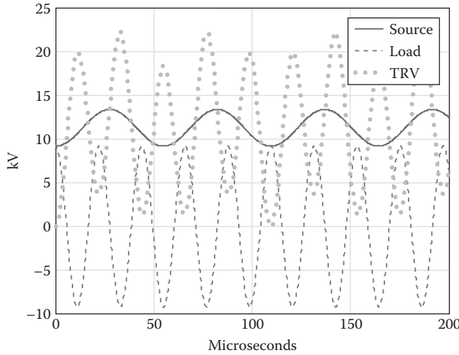
FIGURE 12.7 Double-frequency TRV.
