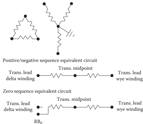
FIGURE 2.18 Transformer equivalent circuit, windings connected delta-wye grounded.
