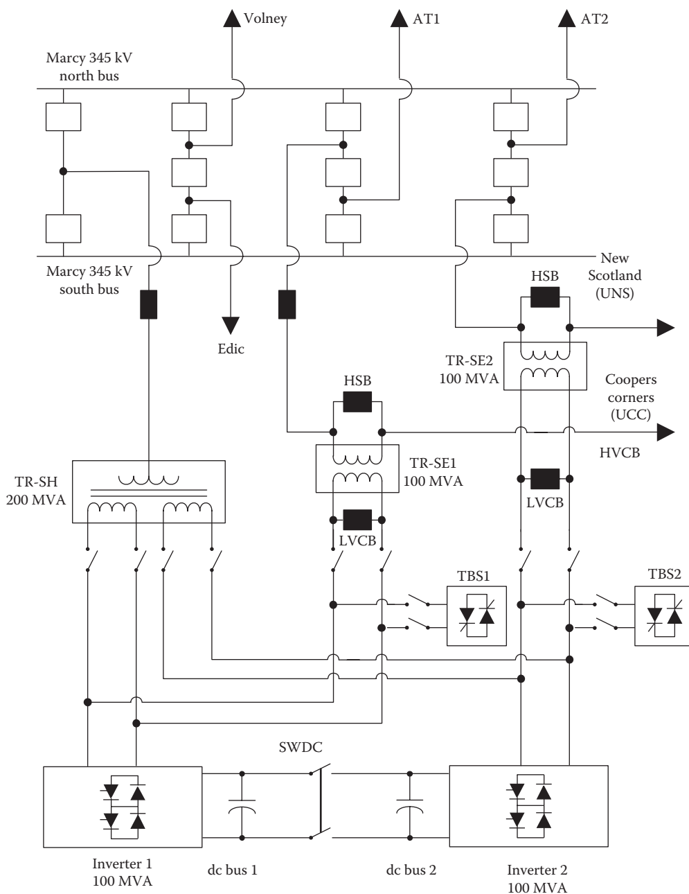
FIGURE 27.50 One-line diagram of 2 \times 100 MVA CSC.
