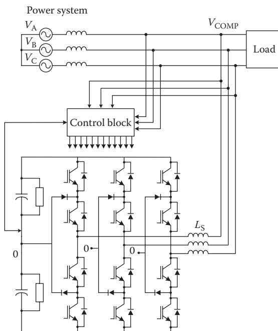
FIGURE 27.15 A STATCOM implemented with a three-level NPC inverter.
