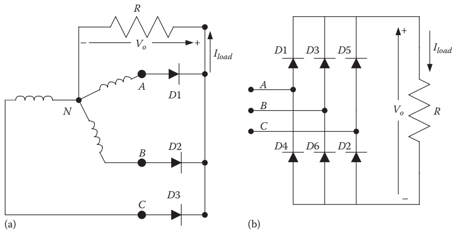
FIGURE 24.12 Schematic representation of three-phase rectifier configurations. (a) Half-wave rectifier needing a neutral point, N ; and (b) full-wave rectifier.
