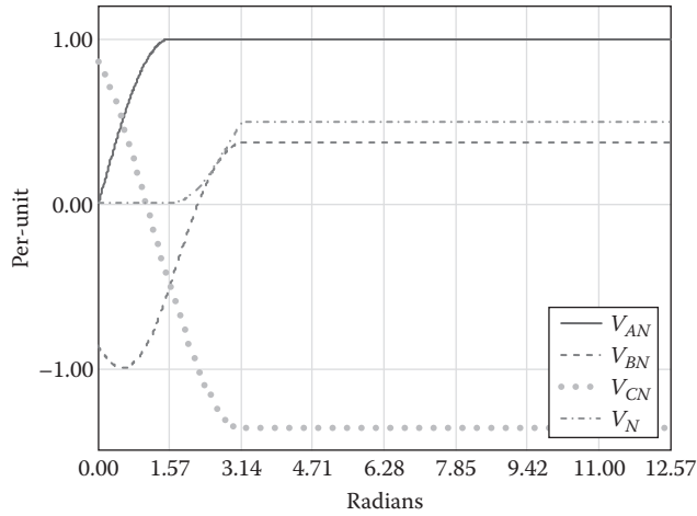
FIGURE 12.13 Ungrounded capacitor bank opening voltages.
