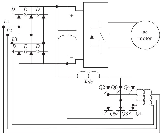
FIGURE 24.38 Use of six-pulse thyristor bridge in the inverter mode to provide regeneration capability to an existing ac drive system.
