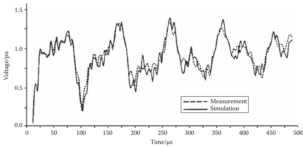
FIGURE 10.7 Comparison of simulation and measurement of disconnect switch-induced overvoltages in a 420 kV GIS. (Copyright 1999 IEEE.)
