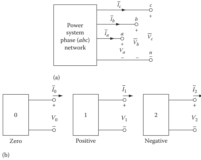
FIGURE 4.4 General fault port in an electric power system. (a) General fault port in phase ( abc ) coordinates; (b) corresponding fault ports in sequence (012) coordinates.
