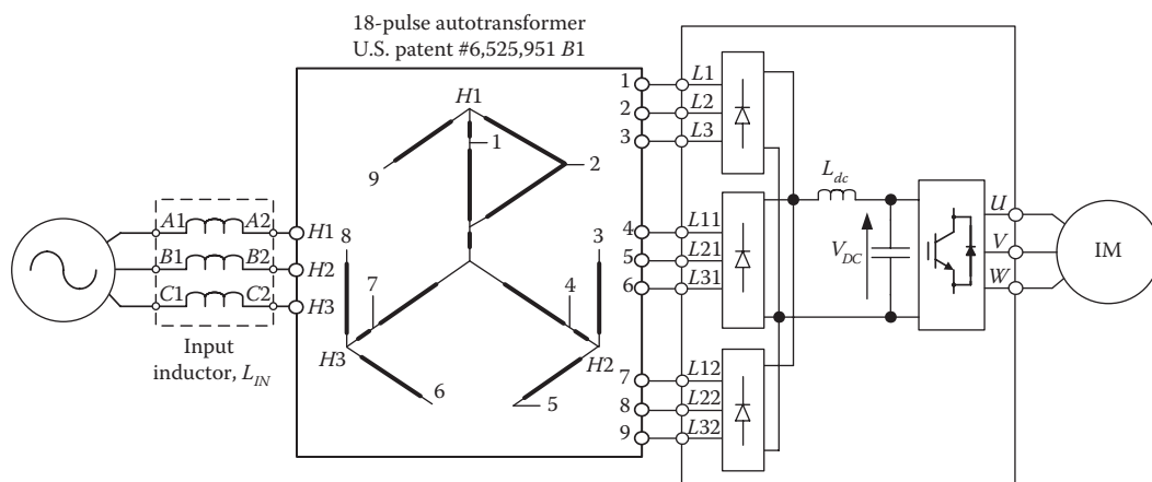
FIGURE 24.29 Schematic of the modified windmill construction of the 18-pulse autotransformer configuration used with VFDs.
