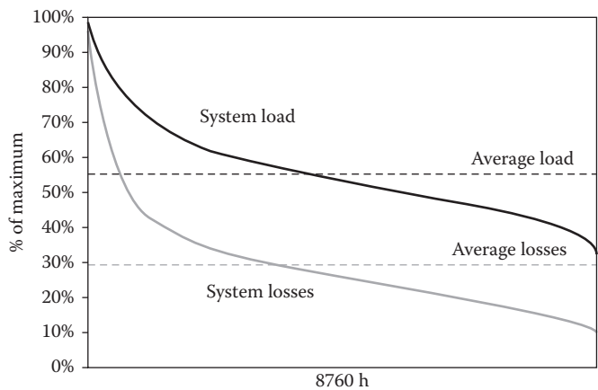
FIGURE 21.7 Annual unitized load duration curves of system load and the associated load-related losses. The LF of the losses is much less than the LF of the load itself as the average losses relative to the peak system losses are much lower. The LFs are equal to the unitized average values.
