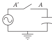
FIGURE 12.8 One phase of grounded capacitor bank opening.
