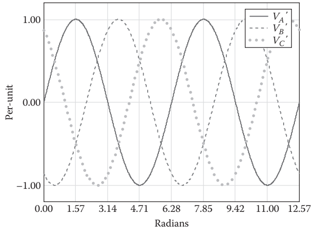
FIGURE 12.11 Ungrounded capacitor bank source voltages.
