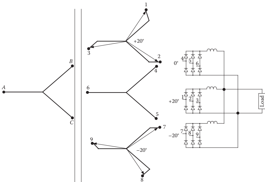
FIGURE 24.27 Schematic representation of 18-pulse converter circuit fed from phase-shifted isolation transformer.
