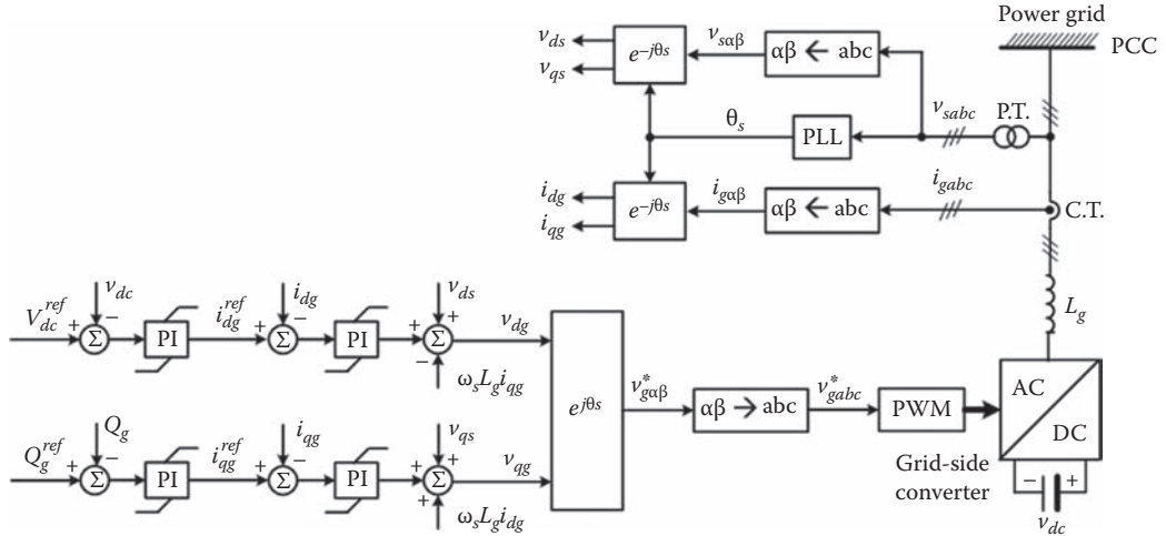
FIGURE 28.17 Synchronous voltage-oriented vector control scheme for the grid-side converter.
