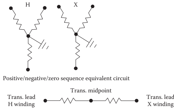
FIGURE 2.17 Transformer equivalent circuit, windings connected wye grounded-wye grounded.
