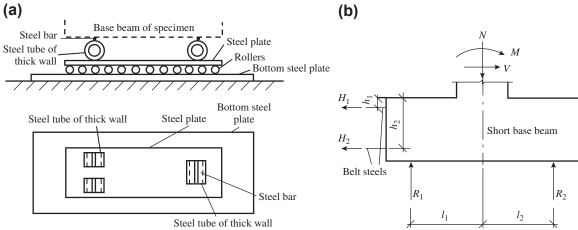
FIGURE 10-6 Roller support with reaction measurement capability and calculation of the internal forces on the bottom section of a column: (a) construction of the roller support; (b) calculation of the internal forces at the bottom of the column.
