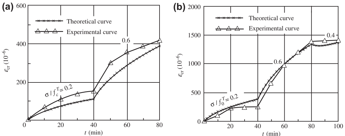
FIGURE 2-15 Short time creep of concrete under constant temperature and variable stress conditions [1-6] : (a) T = 500^\circ\text{C} ; (b) T = 700^\circ\text{C} .
