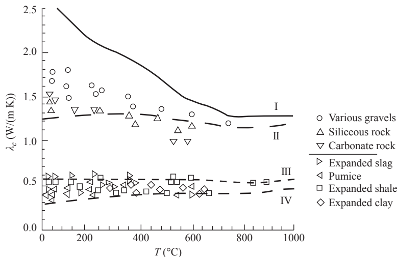
FIGURE 5-6 Coefficient of heat conductivity of concrete with various aggregates [5-2] : siliceous aggregate ( 20^{\circ}\text{C} \leq T \leq 1200^{\circ}\text{C} ).
