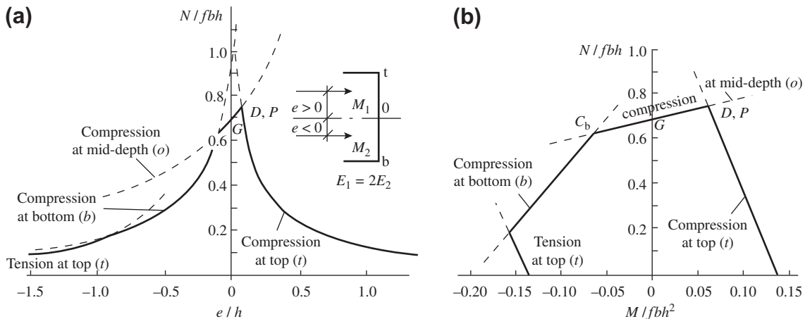
FIGURE 11-6 Ultimate strength of an inhomogeneous linear elastic section: (a) relationship between the ultimate axial compression and eccentricity; (b) ultimate envelope of the axial compression–bending moment.
