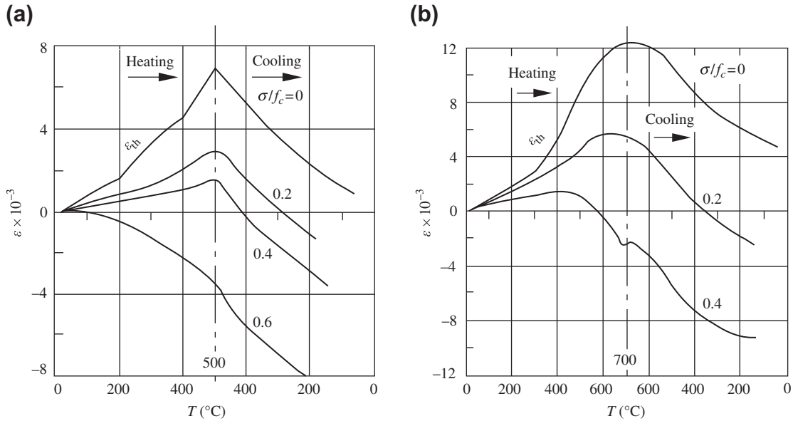
FIGURE 3-9 Heating and cooling strains of concrete under different stress levels [3-5] : (a) T_{\max} = 500\text{ }^{\circ}\text{C} ; (b) T_{\max} = 700\text{ }^{\circ}\text{C} .
