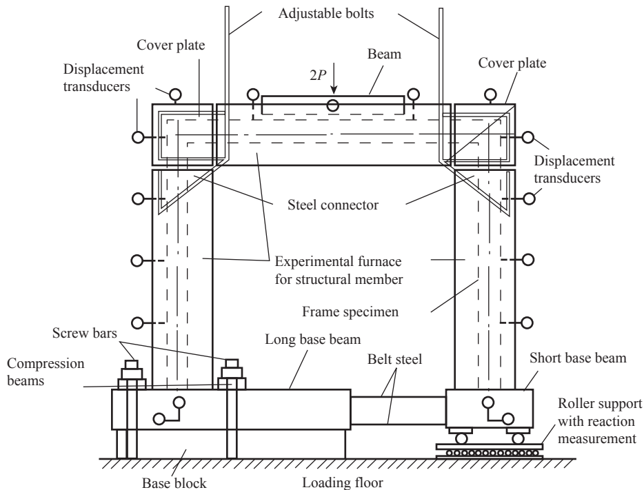
FIGURE 10-5 Experimental devices and measuring points of a frame. [1-12]
