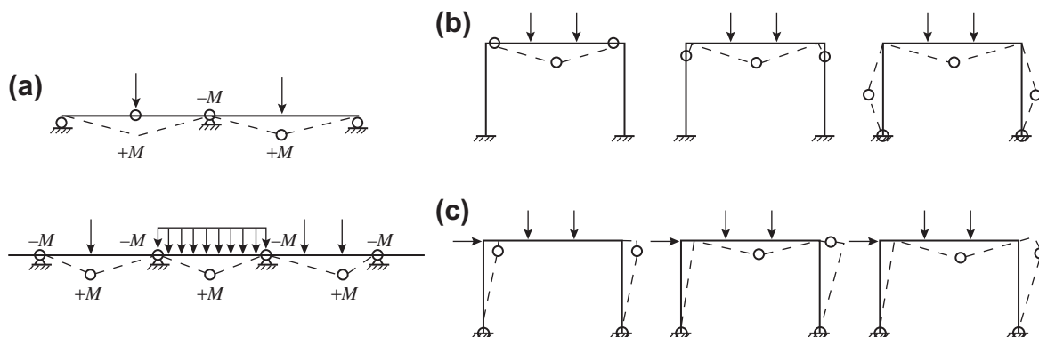
FIGURE 13-11 Possible failure mechanisms of a continuous beam and simple frame: (a) continuous beam; (b) frame (vertical load only); (c) frame (vertical and horizontal loads).
