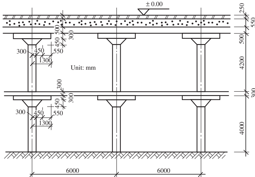
FIGURE 14-1 Size of the slab-column structure in a standard area of an underground building.
