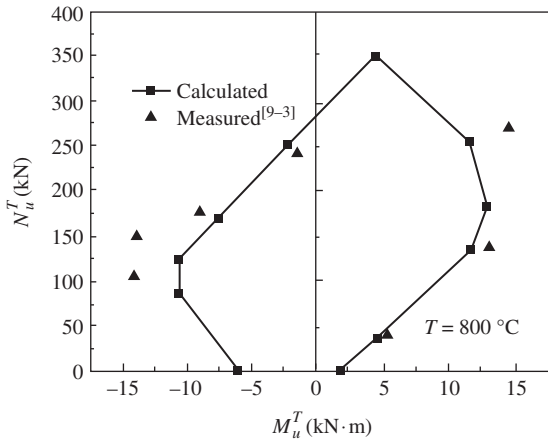
FIGURE 13-10 Demonstration of the calculation method. [13-2]
