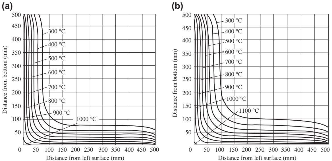
FIGURE 7-19 Temperature contour on a section (500 mm \times 500 mm) of a square column with two adjacent surfaces exposed to fire (a) t = 120 min; (b) t = 180 min.
