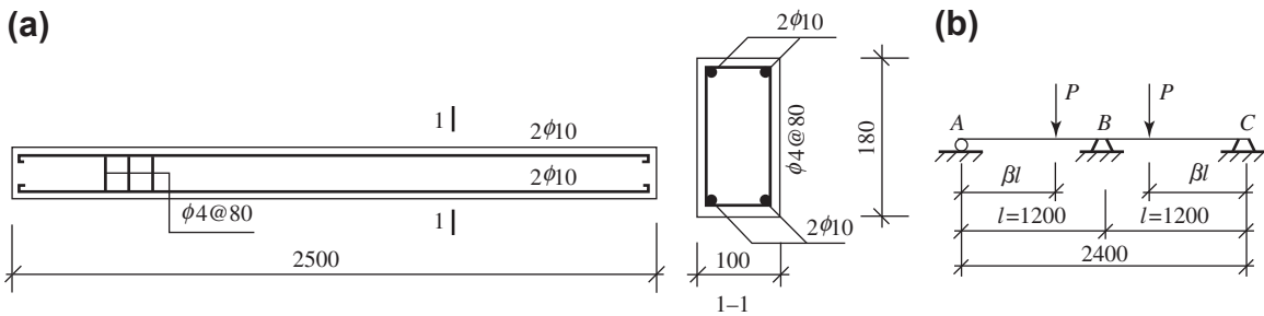
FIGURE 10-1 Construction and loading pattern of a continuous beam specimen [1-12] : (a) specimen; (b) loading pattern.
