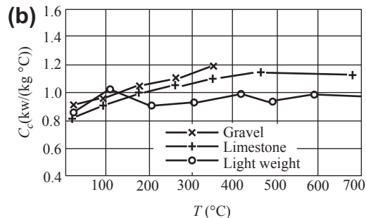
FIGURE 5-8 Specific heat capacity of concrete with different aggregates: (a) from Schneider [5-4] and Harmathy TZ, Allen [5-5] ; (b) from Federation International de la Précontrainte. [5-7]
