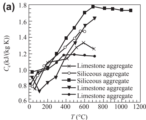
FIGURE 5-8 Specific heat capacity of concrete with different aggregates: (a) from Schneider [5-4] and Harmathy TZ, Allen [5-5] ; (b) from Federation International de la Précontrainte. [5-7]
