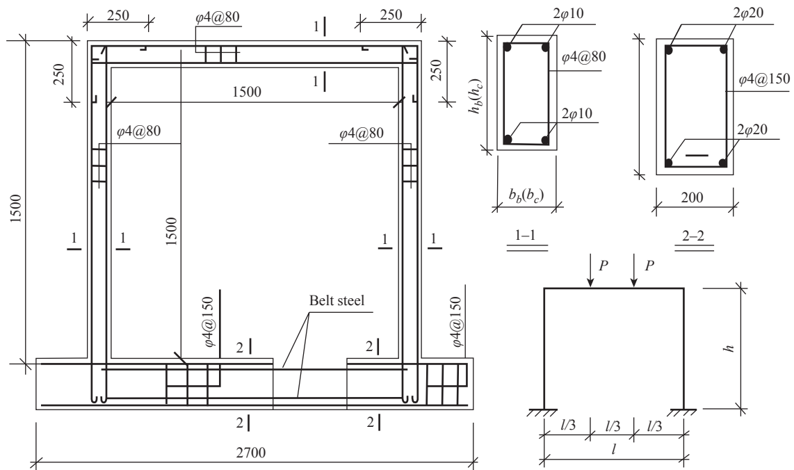
FIGURE 10-2 Construction and loading pattern of a frame specimen. [11-12]
