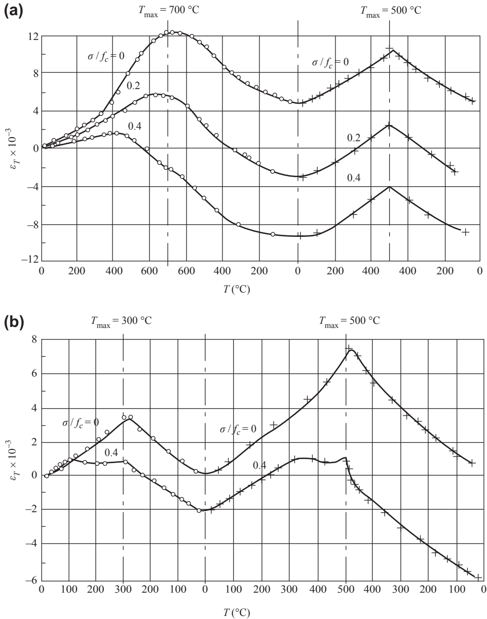
FIGURE 3-12 Thermal strain of concrete during multicycles of heating-cooling [3-5] : (a) 700–500 ^{\circ}\text{C} ; (b) 500–700 ^{\circ}\text{C} .
