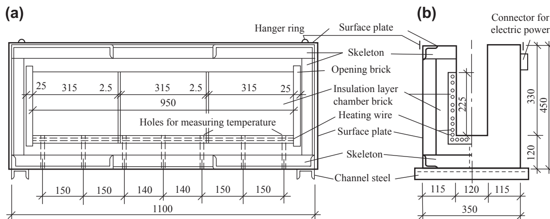
FIGURE 8-3 Construction of a furnace for testing members [1-12] : (a) longitudinal section; (b) transverse section.
