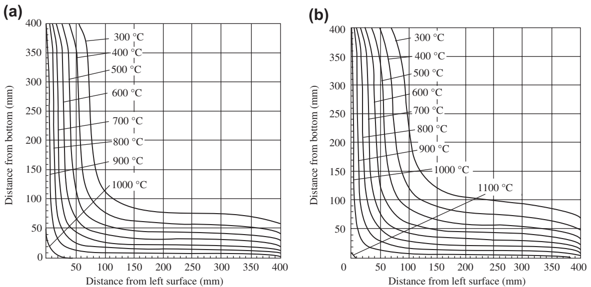
FIGURE 7-18 Temperature contour on a section (400 mm x 400 mm) of a square column with two adjacent surfaces exposed to fire: (a) t = 120 min; (b) t = 180 min.
