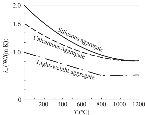
FIGURE 5-7 Calculated value of the coefficient of heat conduction of concrete. [2-6]
