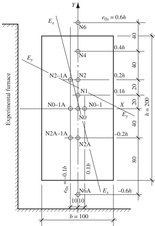
Figure 9-21 Initial positions of the load for all specimens. [9-6]
