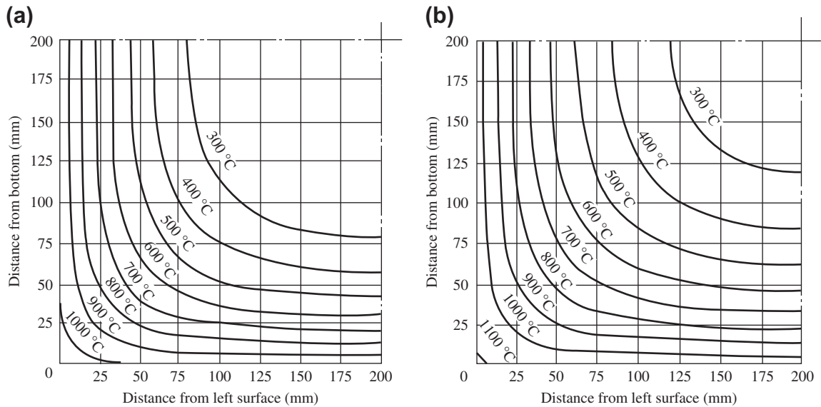
FIGURE 7-13 Temperature contour on a section (400 mm \times 400 mm) of a square column with four surfaces exposed to fire: (a) t = 120 min; (b) t = 180 min.
