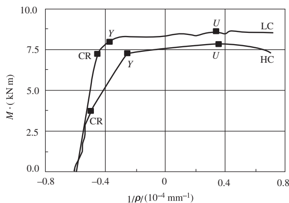
FIGURE 8-14 Bending moment–curvature relationship for beams with the compression zone exposed to a high temperature. [8-14]
