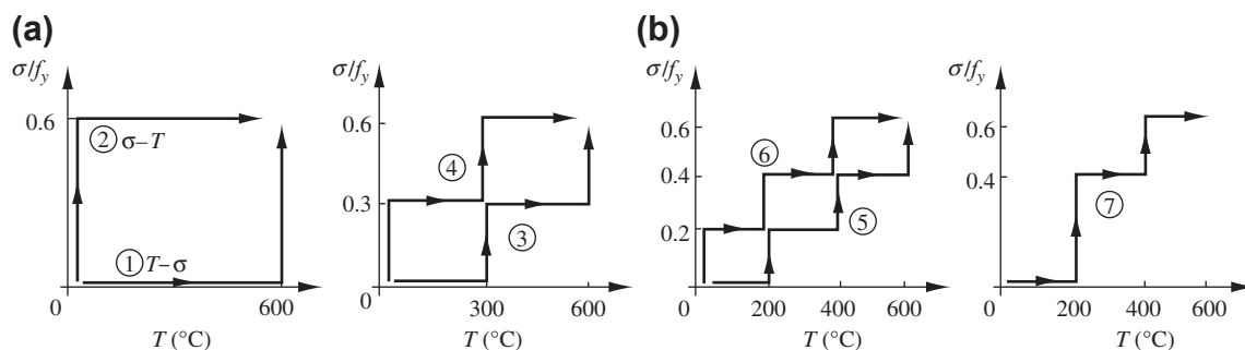
Figure 4-8 Various temperature–stress paths for testing reinforcement [4-1] : (a) extreme paths; (b) complicated paths.
