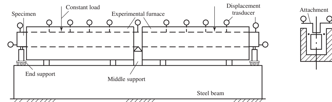
FIGURE 10-3 Experimental devices and measuring points for a continuous beam. [1-12]
