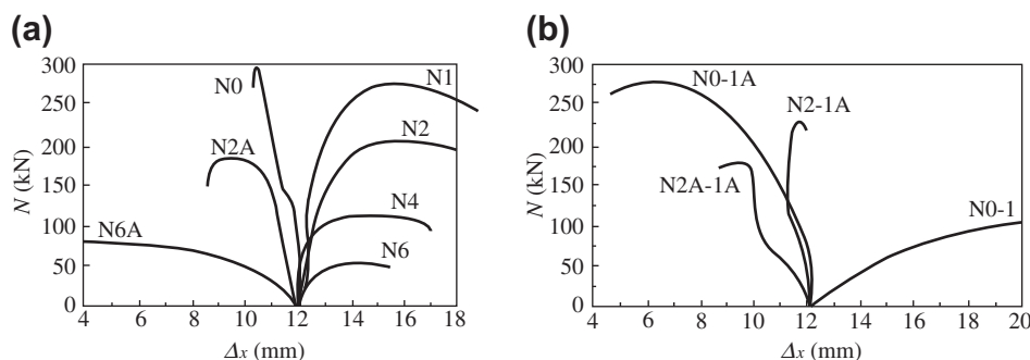
Figure 9-25 Horizontal deflection of eccentric compressive specimens with two adjacent surfaces exposed to high temperature [9-6] : (a) e_{0x} = 0 , e_{0y} \neq 0 ; (b) e_{0x} \neq 0 , e_{0y} = 0 .
