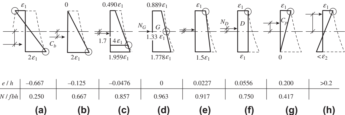
FIGURE 11-9 Various conditions of mechanical character of a section with continuously variable behavior. Solid line, strain on section; dashed line, ultimate strain of material; circle, failure control point.
