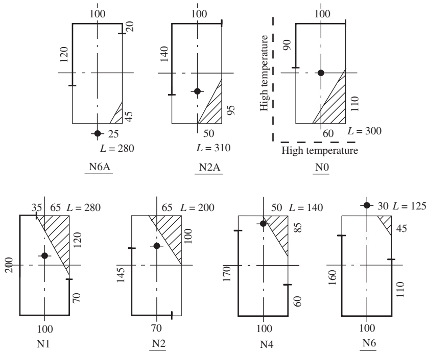
Figure 9-28 Failure zone on the section of a compressive specimen with two adjacent surfaces exposed to high temperature and with one-directional eccentricity ( e_{ox} = 0 ) only. [9-14] The black dot in this figure shows the initial position of the load, the shaded area represents the compression failure zone, L is the longitudinal length of the compression failure zone, and the thick lines along the periphery denote the scope of the tensile crack and the figure noted shows the length along the periphery of the section.
