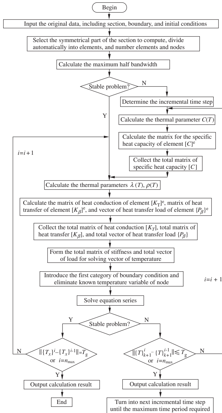
FIGURE 6-10 Flow chart for the HTARC program.
