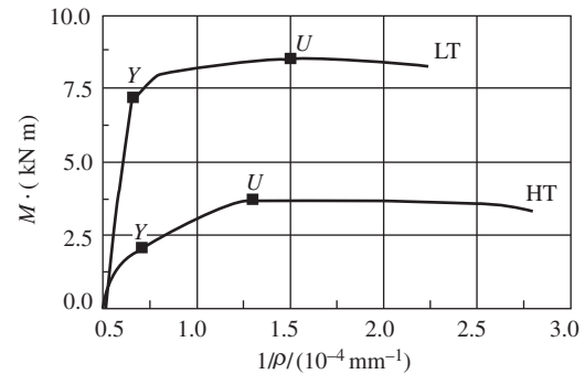
FIGURE 8-13 Bending moment–curvature relationship for beams with the tension zone exposed to a high temperature. [8-14]
