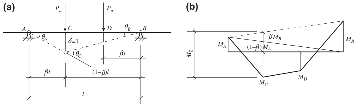
FIGURE 13-12 Calculation model of the ultimate load of a continuous beam: (a) failure mechanism and virtual displacement; (b) bending moment diagram at the ultimate state.
