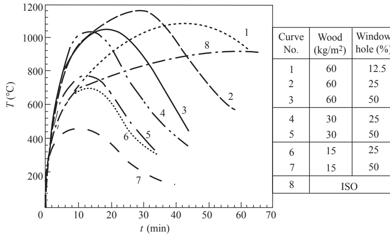
FIGURE 5-2 Experimental temperature–time curves of wood burning. [0-13]
