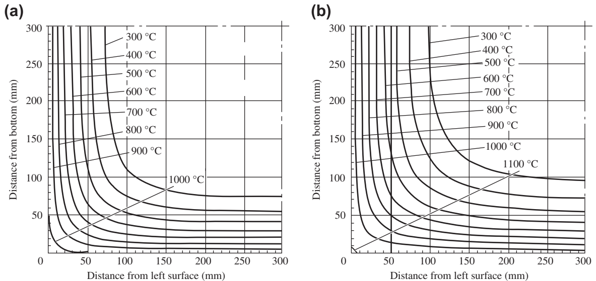
FIGURE 7-14 Temperature contour on a section (500 mm \times 500 mm) of a square column with four surfaces exposed to fire: (a) t = 120 min; (b) t = 180 min.
