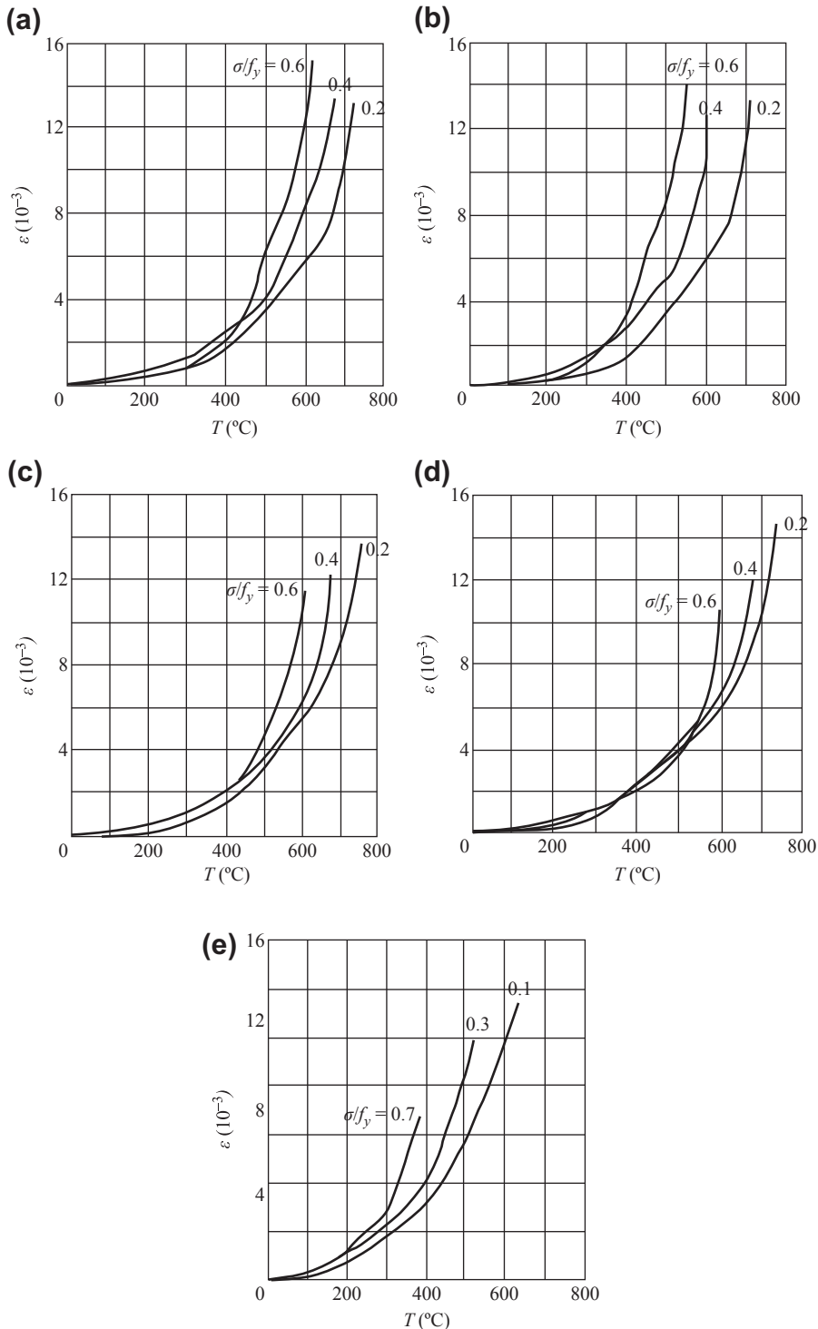
Figure 4-14 Thermal strain of reinforcement under the action of stress [4-11] : (a) steel grade I; (b) steel grade II; (c) steel grade III; (d) steel grade IV; (e) steel grade V.
